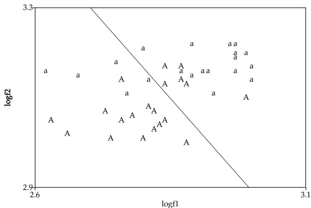
Figure 3.2: Regression boundary obtained for the data of the pretest, together with the positions of the stimuli with respect to logf1 and logf2. (A= /a/ and a=/a:/).
