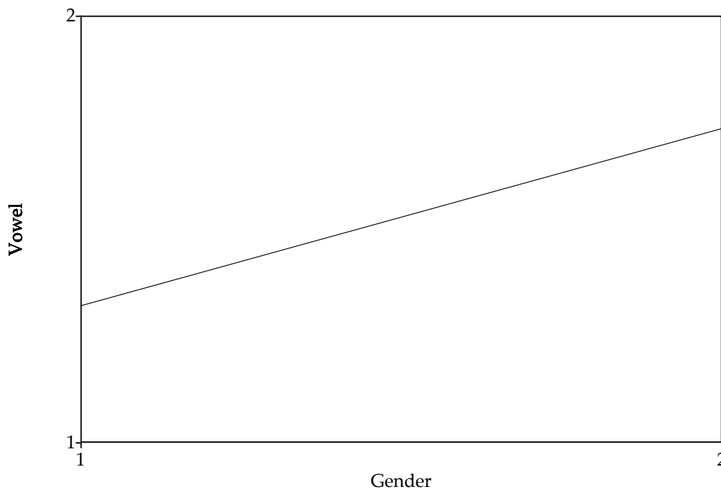
Figure 3.1: Regression line obtained for the data of the present example (Spanish-speaking subjects, enhanced condition, pretest). Gender (1 = female, 2 = male), Vowel (1 = / \alpha /, 2 = / a: /).
