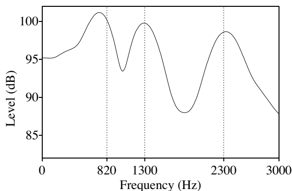
Figure 7: Truncated-filter spectrum.
